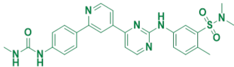
hSMG-1 inhibitor 11e 1402452-10-1
